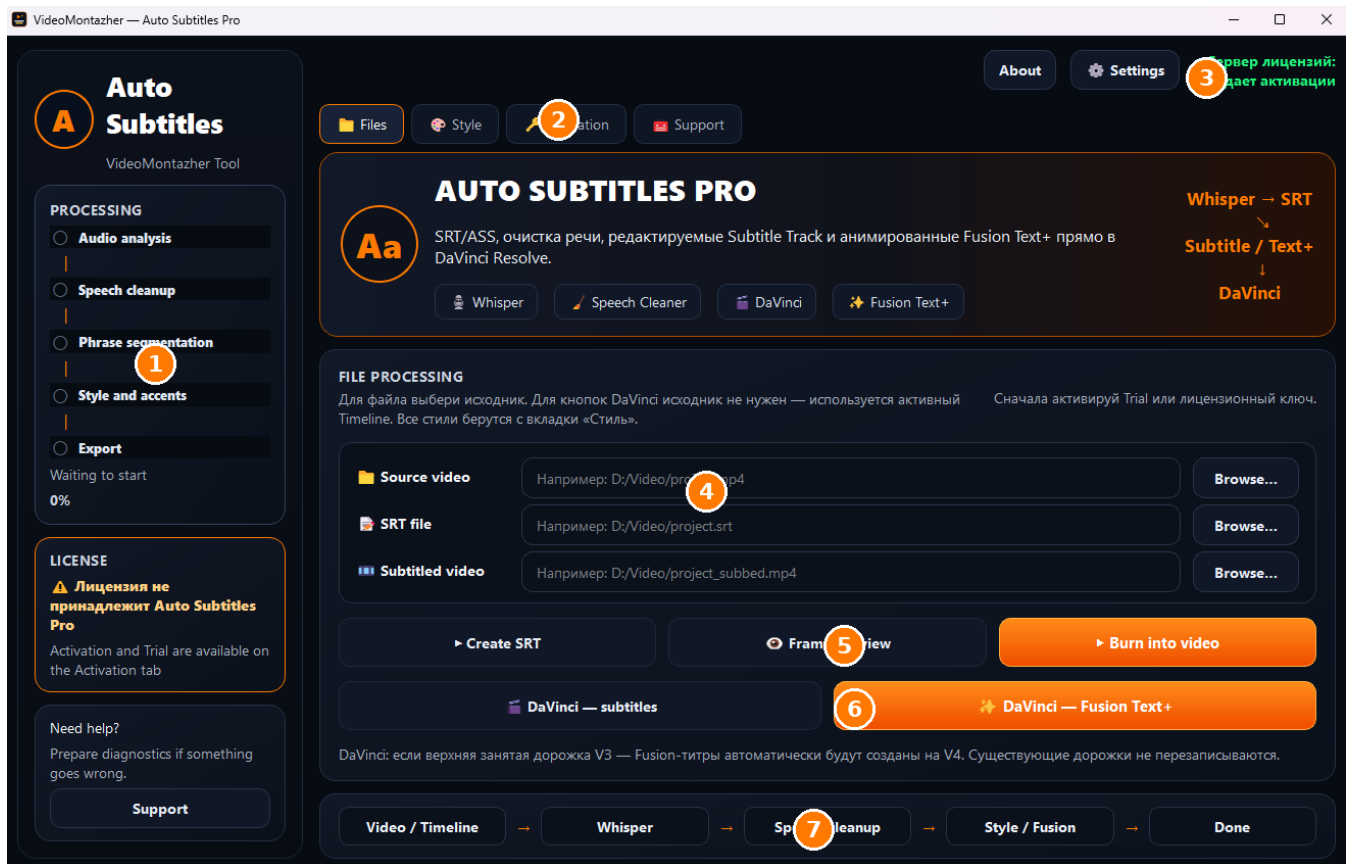
Main screen. 1 - processing stages, 2 - tabs, 3 - license status, 4 - file paths, 5 - file actions, 6 - DaVinci actions, 7 - pipeline.
